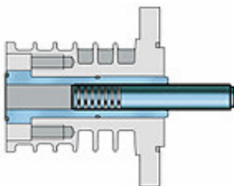
High performance final stage piston
